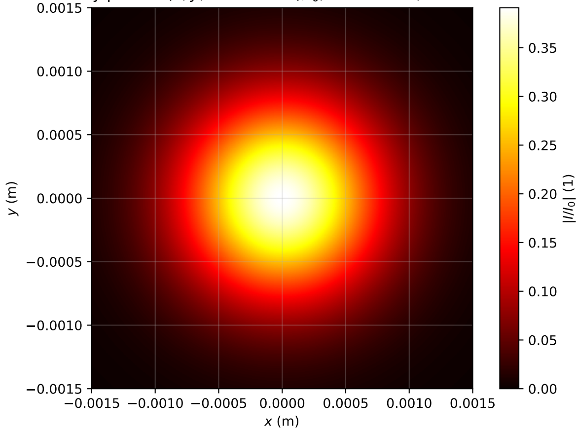
Intensity profile I(x, y, z = 3.184m)/I_0 , P_{in}=0.3P_{cr} , artificial time
